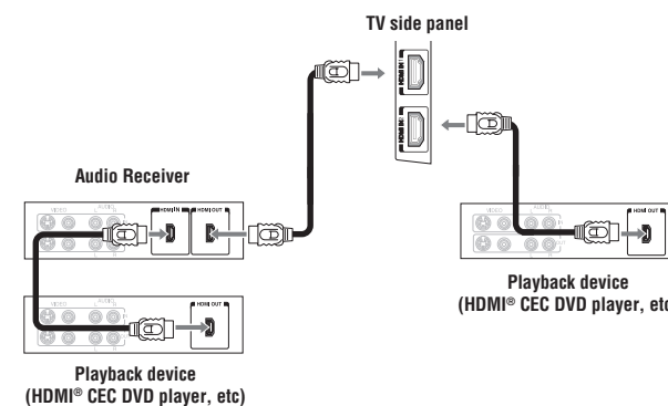
(Sample Illustration) Connecting HDMI® CEC compatible audio receiver and playback device connections
