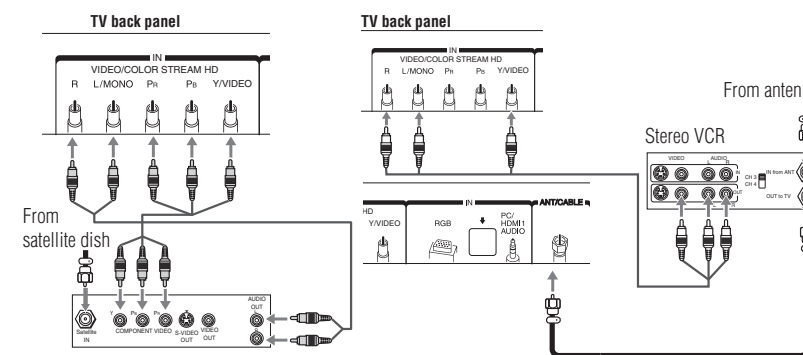
(Sample Illustration) Connecting a Blu-ray™/DVD player, satellite receiver, or VCR with ColorStream®
