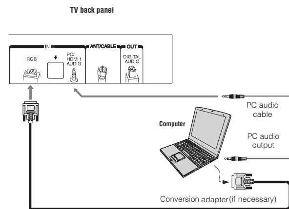
(Sample Illustration) Connecting a computer
