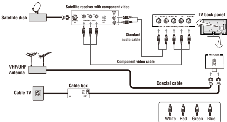
(Sample Illustration) L7350U Series—Connecting to an antenna, satellite receiver, and/or cable TV box
